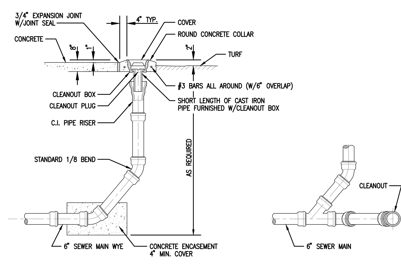
TYPICAL EXTERIOR CLEANOUT DETAIL NOT TO SCALE
