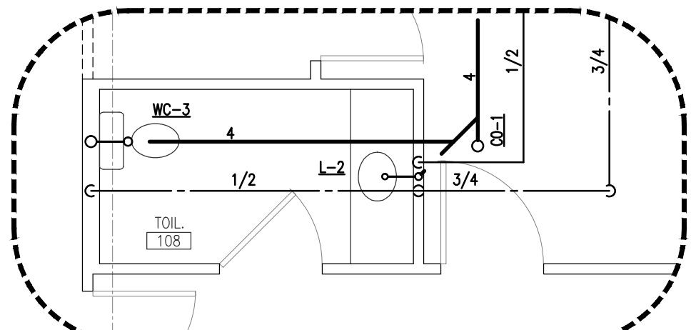
ENLARGED TOILET 108 PLAN SCALE: 1/4" = 1'-0"
