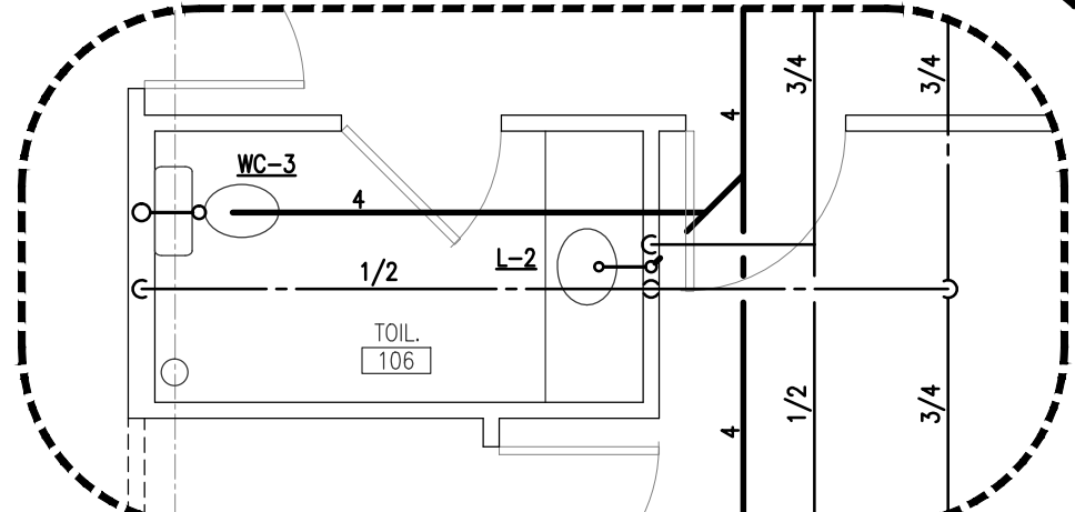
ENLARGED TOILET 106 PLAN SCALE: 1/4" = 1'-0"
