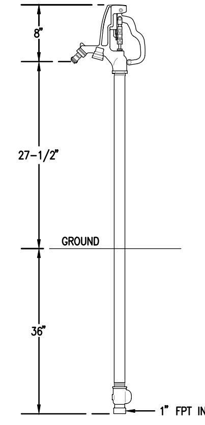
WOODFORD Y2 YARD HYDRANT DETAIL NOT TO SCALE
