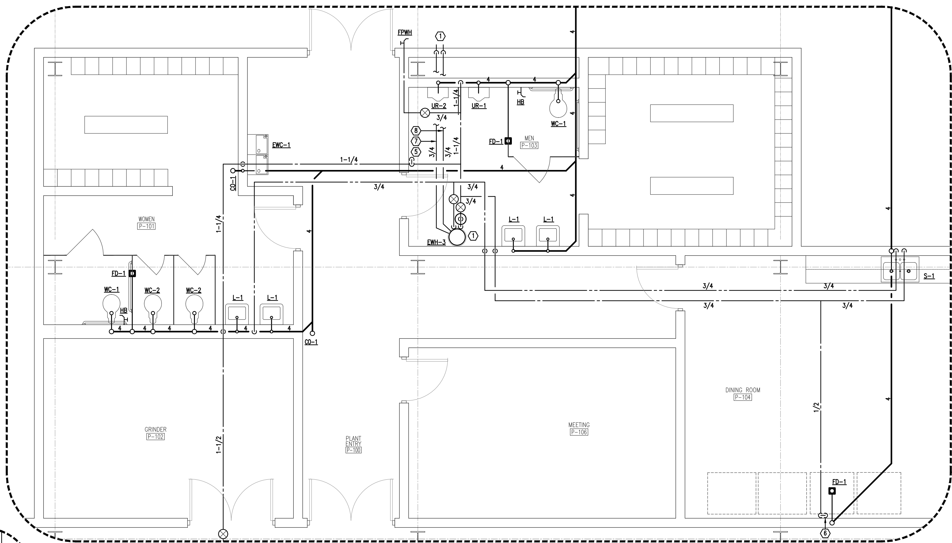
ENLARGED RESTROOM P-101 & P-103, & DINING ROOM P-104 PLAN SCALE: 1/4" = 1'-0"
