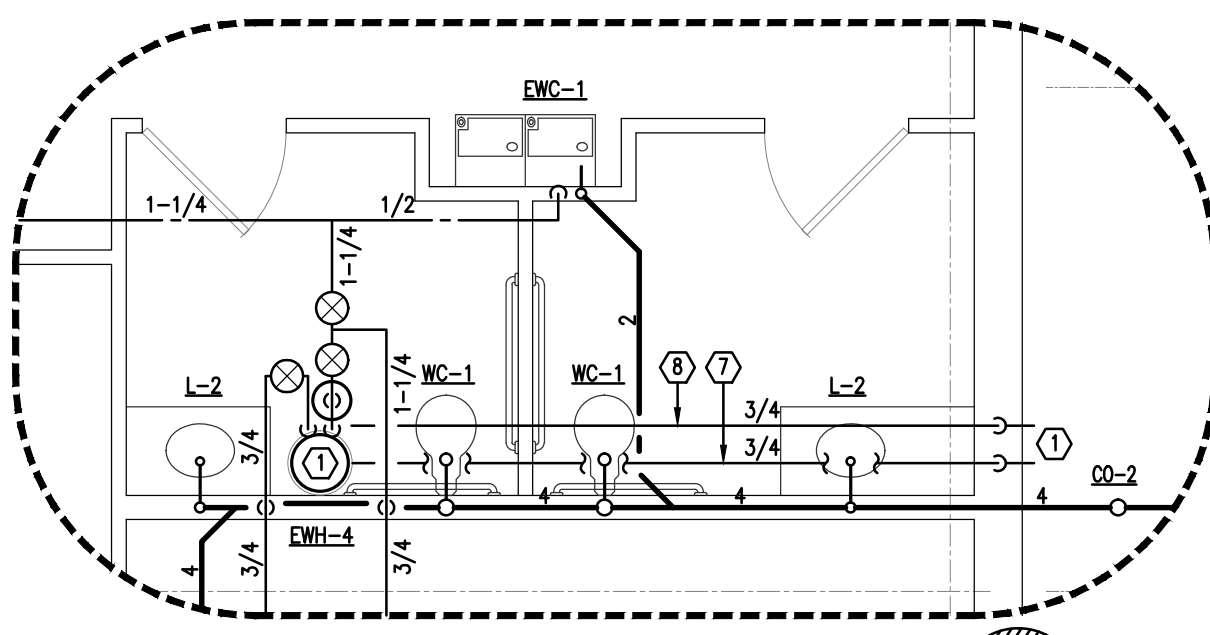
ENLARGED RESTROOM 101 & 102 PLAN SCALE: 1/4" = 1'-0"
