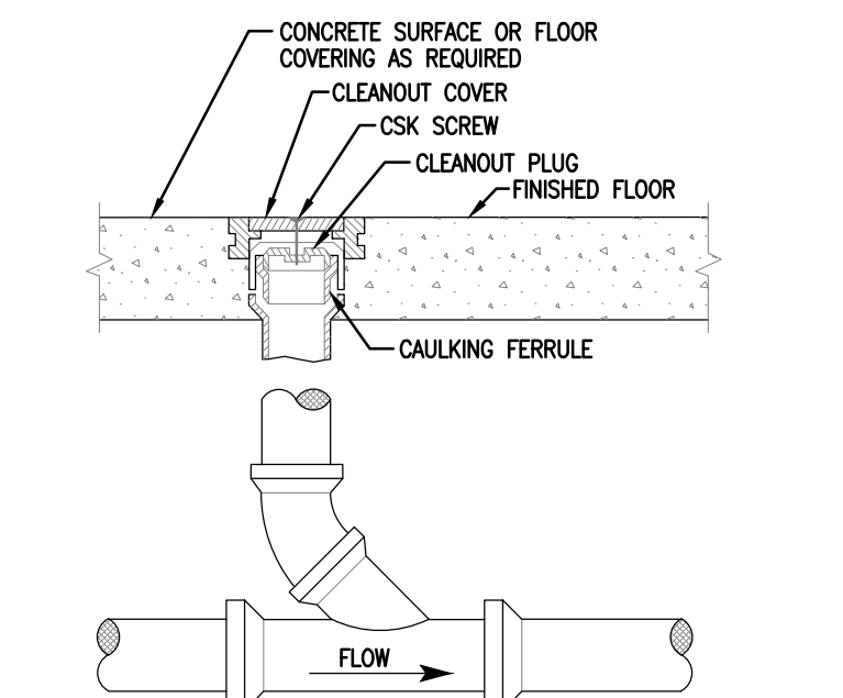
FLOOR CLEANOUT-FINISHED ROOM NOT TO SCALE
