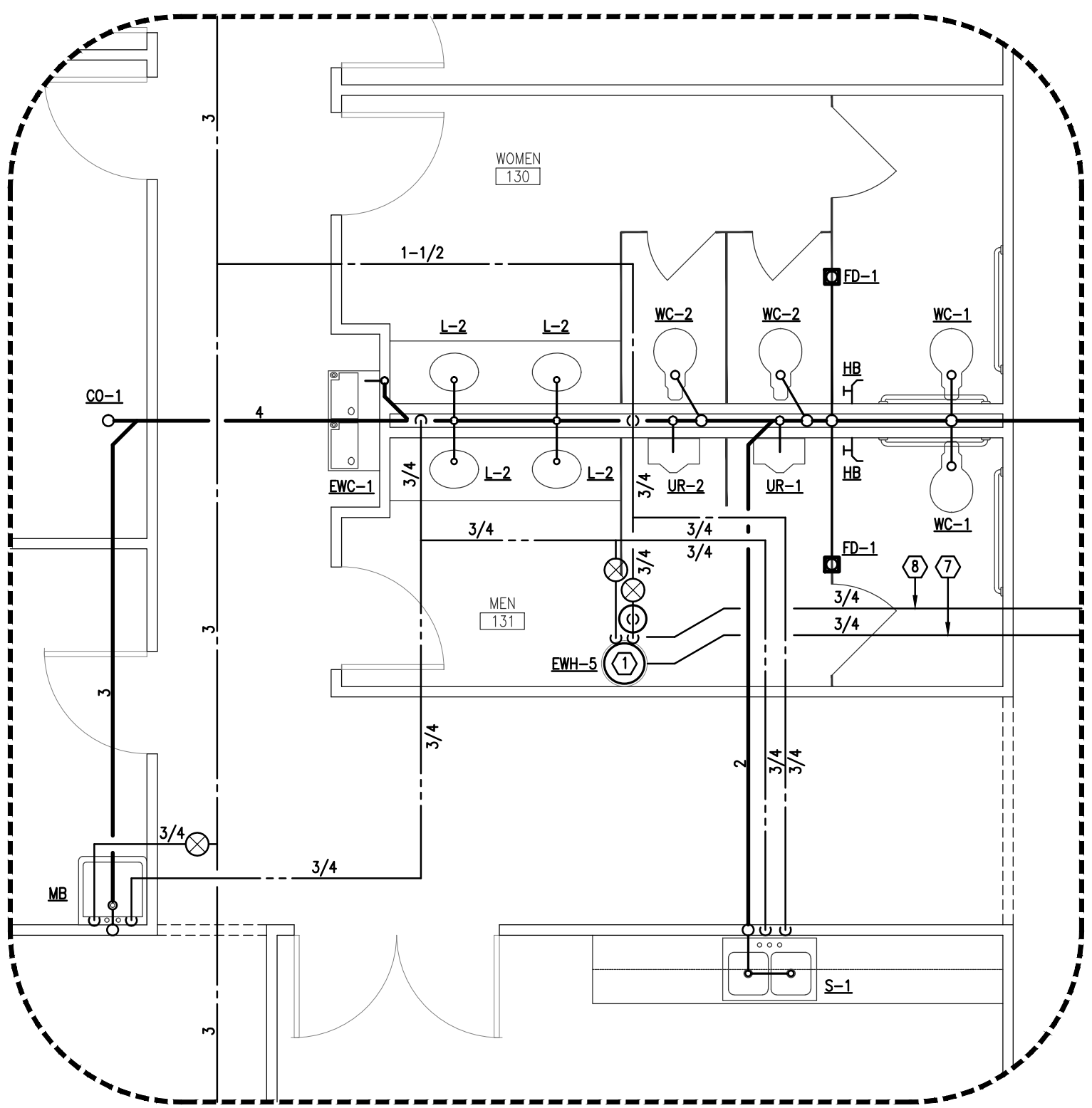
ENLARGED RESTROOM 130 & 131 PLAN SCALE: 1/4" = 1'-0"
