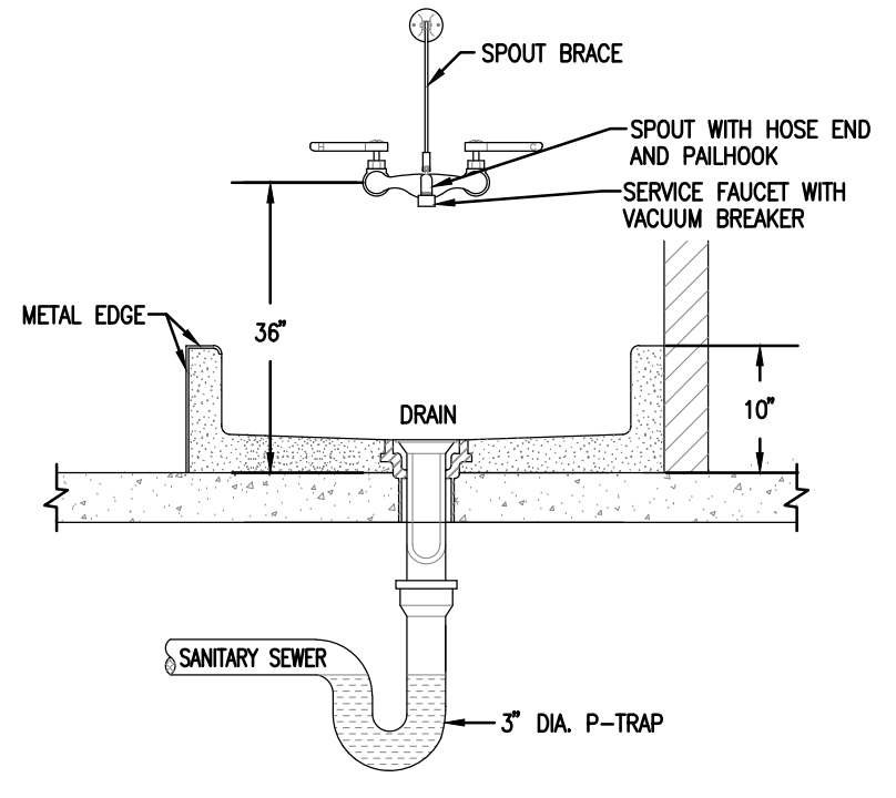
MOP SINK DETAIL NOT TO SCALE
