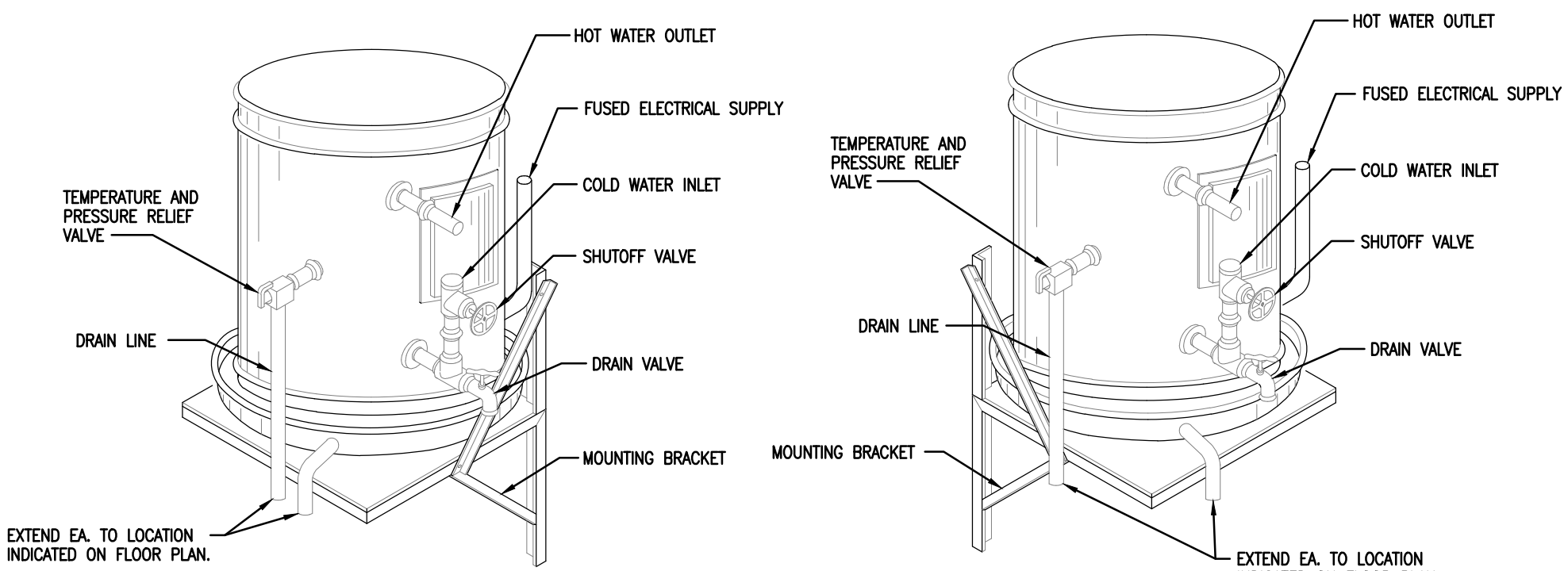
WALL MOUNTED ELECTRIC WATER HEATER NOT TO SCALE
