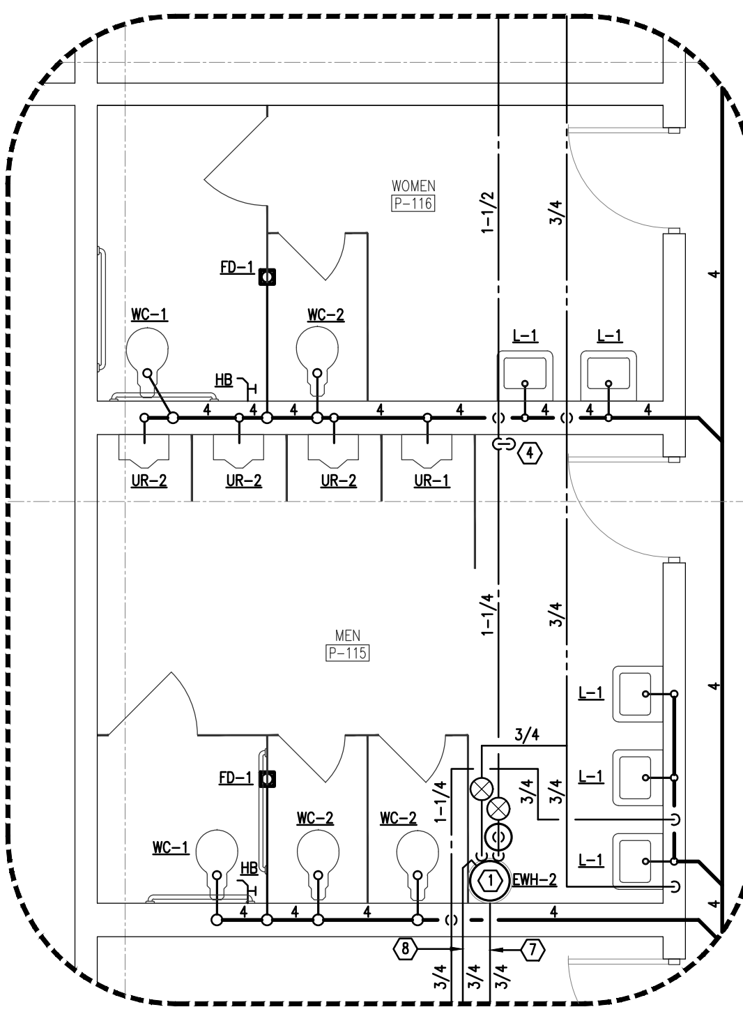
ENLARGED RESTROOM P-115 & P-116 PLAN SCALE: 1/4" = 1'-0"
