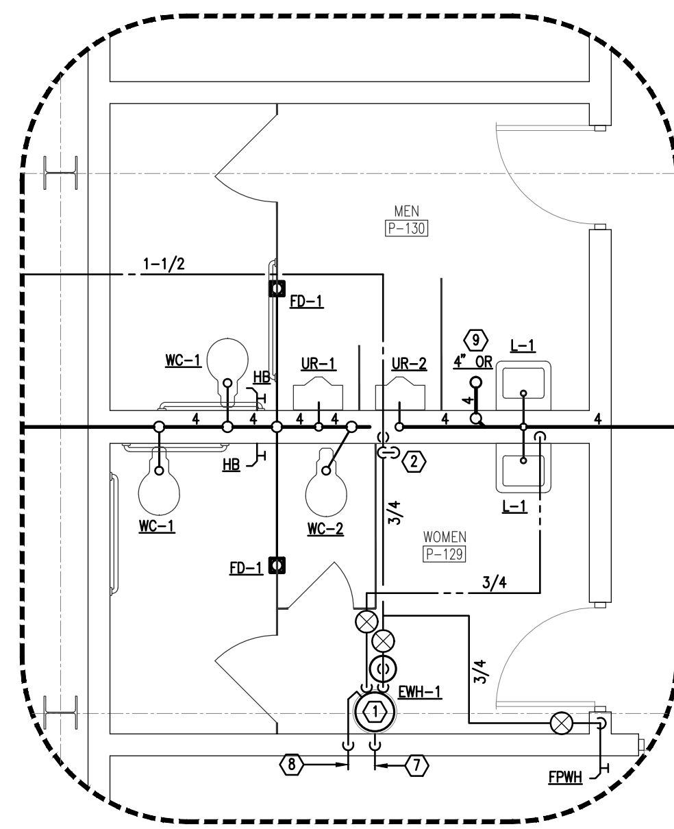
ENLARGED RESTROOM P-129 & P-130 PLAN SCALE: 1/4" = 1'-0"
