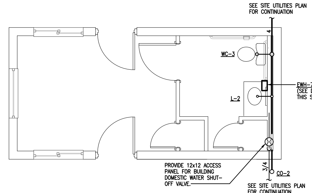
GUARD SHACK PLUMBING FLOOR PLAN SCALE: 1/4" = 1'-0"
