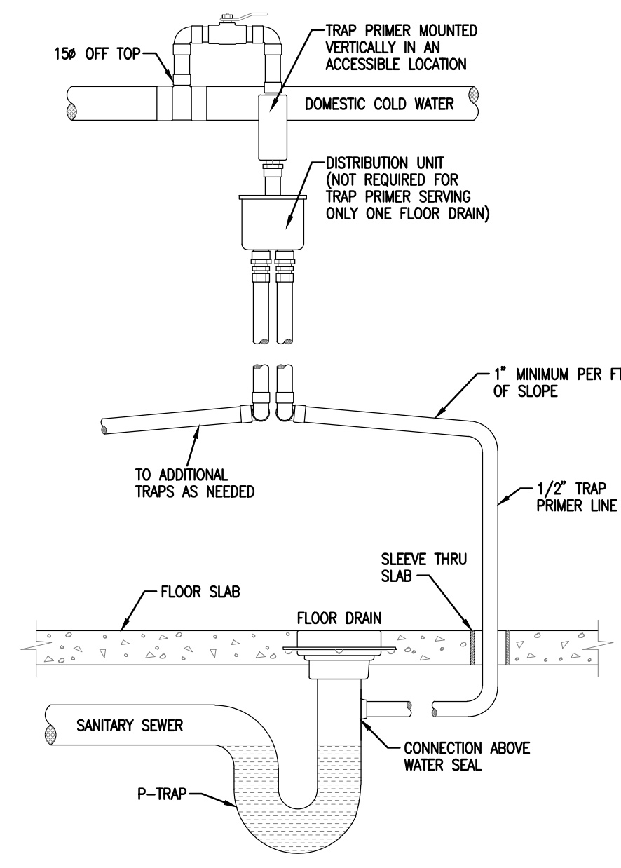
TYPICAL TRAP PRIMER DETAIL NOT TO SCALE
